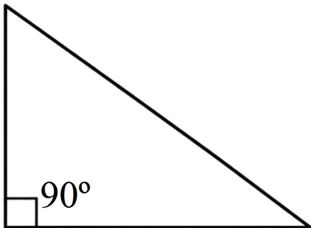
Right Triangle
