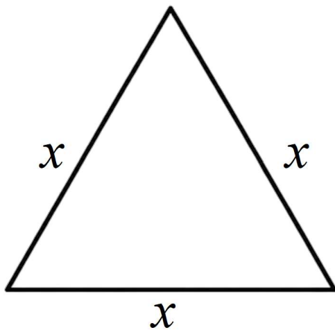
Equilateral Triangle
