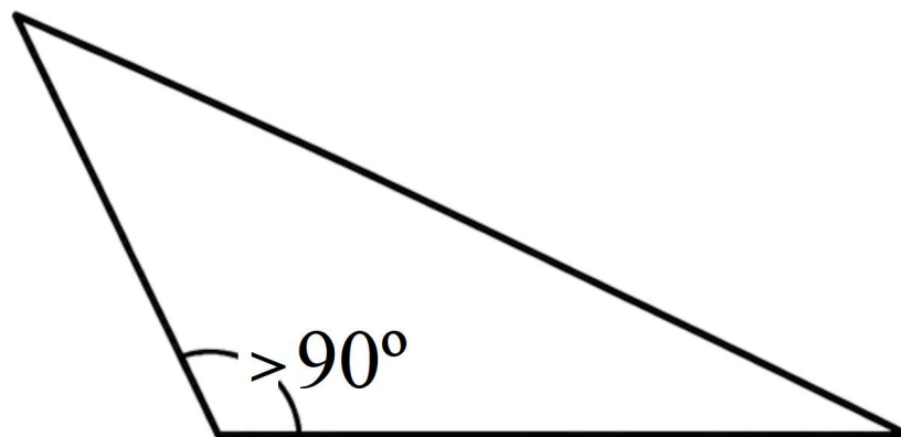
Obtuse Triangle
