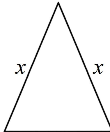
Isosceles Triangle
